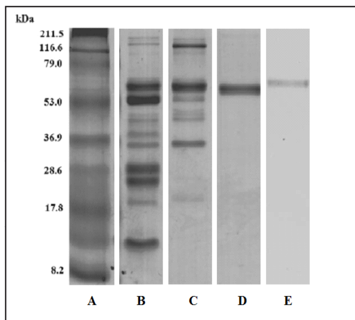
FIGURE 5. Porthidium l. hutmanni SDS-PAGE. A) molecular weight markers; B) crude venom; C) FI; D) hutmannin-1 under native conditions; E) hutmannin-1 under reduction conditions. All samples were run with 25 \mu g of protein.
