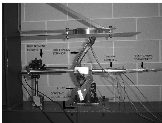
FIGURE 2. SPECIMEN ASSEMBLY PRIOR TO THE TRIALS AND MEASURING SYSTEMS (ON THE LEFT OF SPECIMEN DISPLACEMENT SENSORS AND ON THE RIGHT, FORCE SENSOR).
